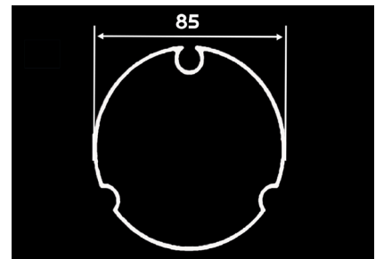
CODE: 34002 85 MM ALÜMİNYUM BORU
