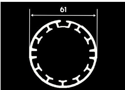
CODE: 34339 61 MM ALÜMİNYUM BORU
