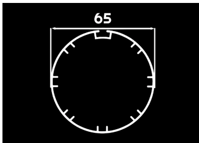
CODE: 34226 65 MM ALÜMİNYUM BORU
